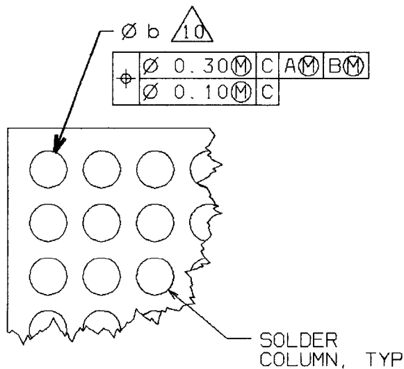
DETAIL A
