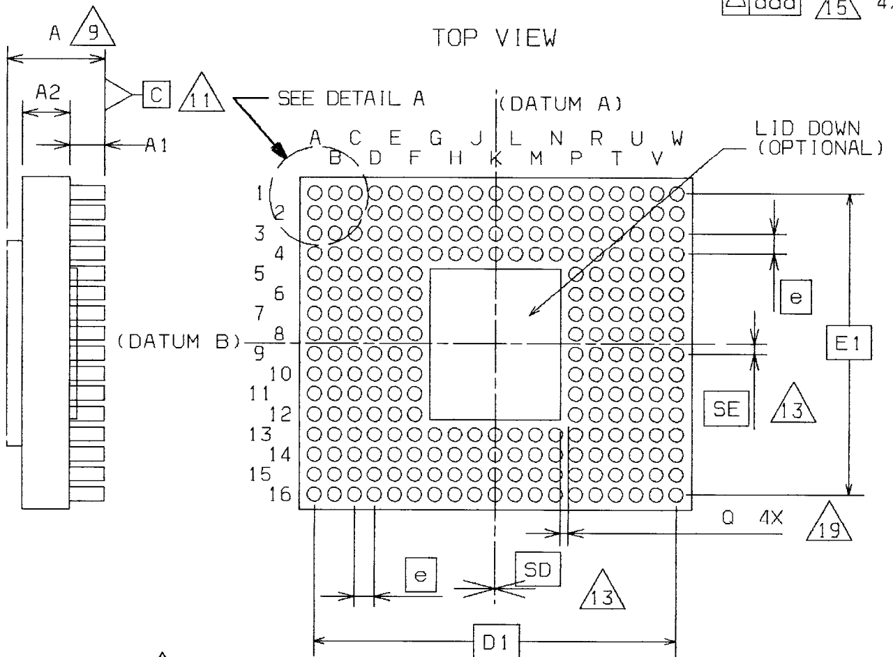
BOTTOM VIEW
