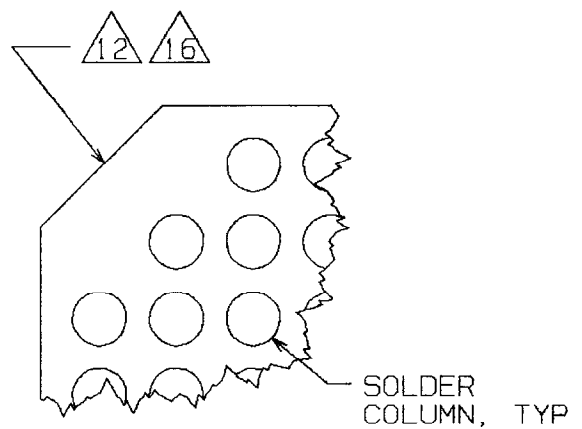
DETAIL A CORNER A1 OPTIONAL CONFIGURATION
